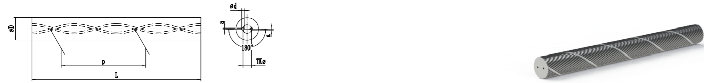
Unground Rods with 2 Helix Coolant Holes 30°
