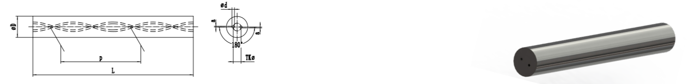
Ground Rods with 2 Helix Coolant Holes 30°
